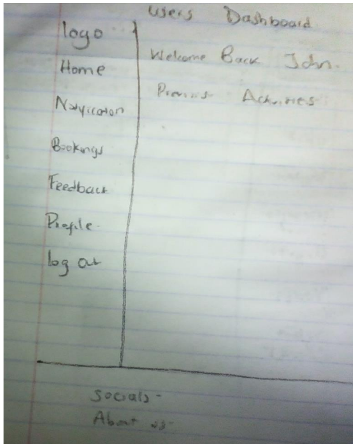
Figure 6. Users dashboard
