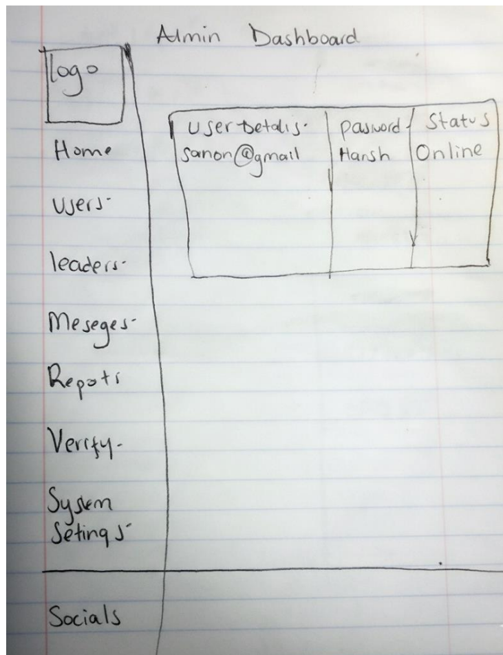
Figure 7. Administrator dashboard.
