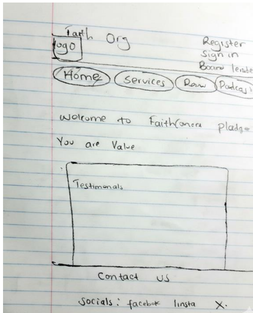
Figure 1.Home page layout
